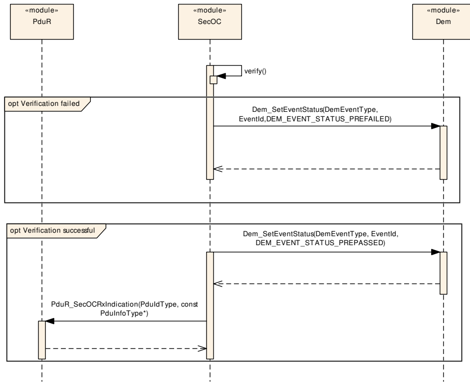
Figure 9.8: SecOC verification reporting to Dem
