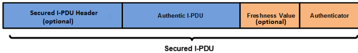
Figure 7.2: Secured I-PDU contents
