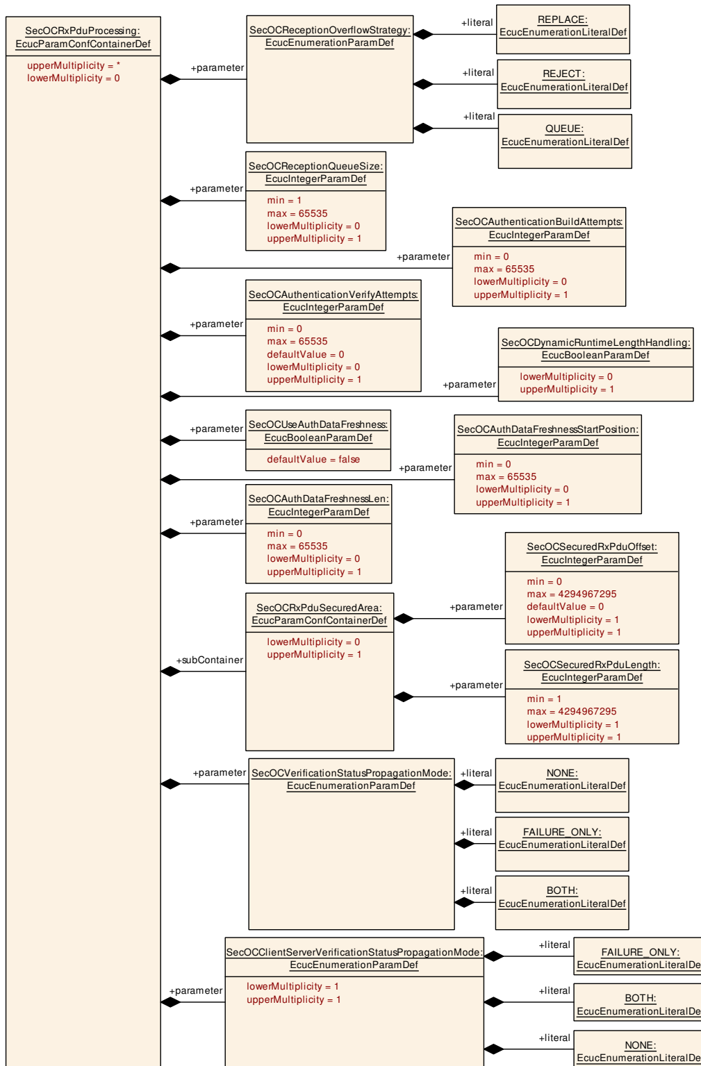
Figure 10.3: The AUTOSAR SecOC Rx Pdu Configuration Part 2
