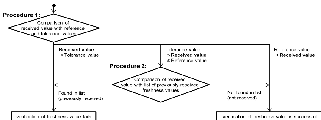
Figure A.12: Verification of freshness value
