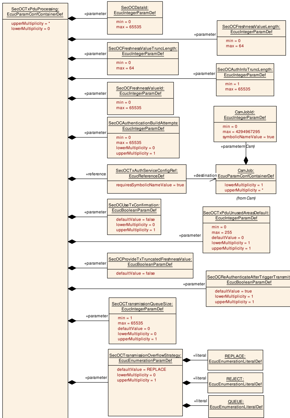
Figure 10.5: The AUTOSAR SecOC Tx Pdu Configuration Part 2
