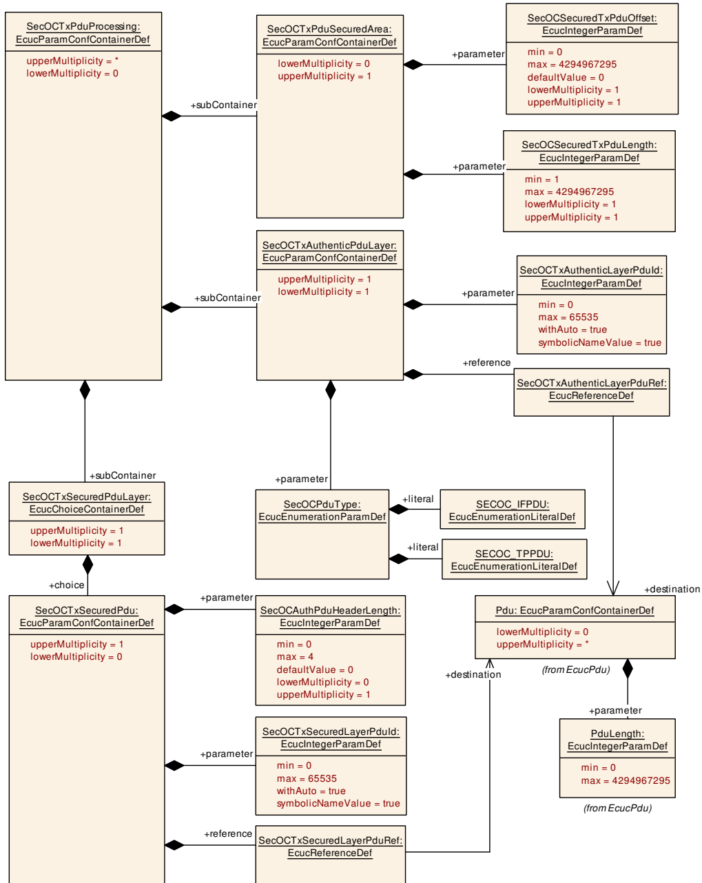
Figure 10.4: The AUTOSAR SecOC Tx Pdu Configuration Part 1
