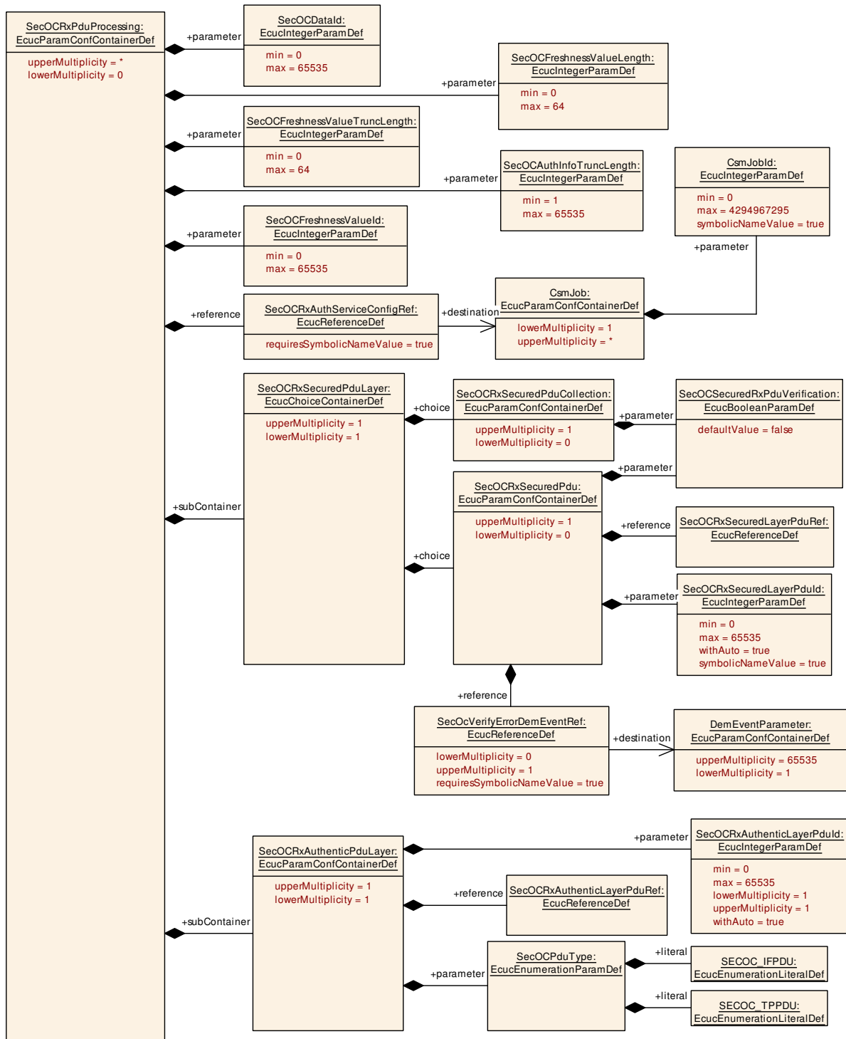
Figure 10.2: The AUTOSAR SecOC Rx Pdu Configuration Part 1
