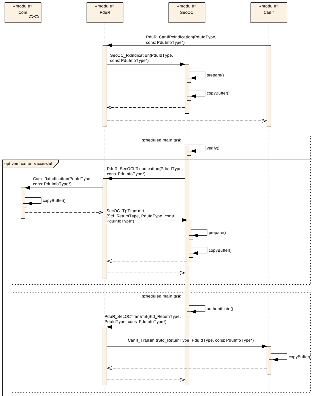
Figure 9.9: Verification and authentication in a gateway situation
